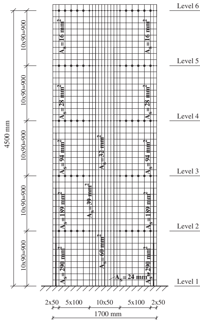
Figure 8. Finite element model for spectral analysis
