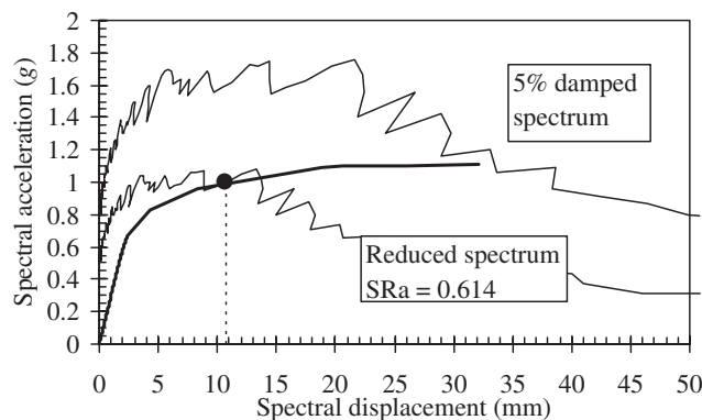
Figure 9. Response spectra to 15 mm performance for Nice record (PGA 0.61 g)
