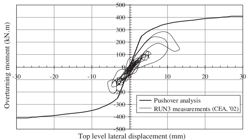
Figure 7. Comparison between the pushover analysis and RUN3 measurements (CEA, 2002) moment-displacement relationships
