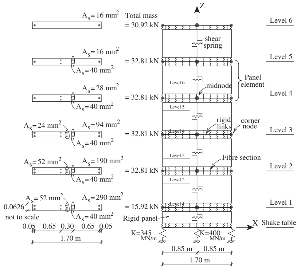
Figure 12. Properties of the modeled wall for time history analysis
