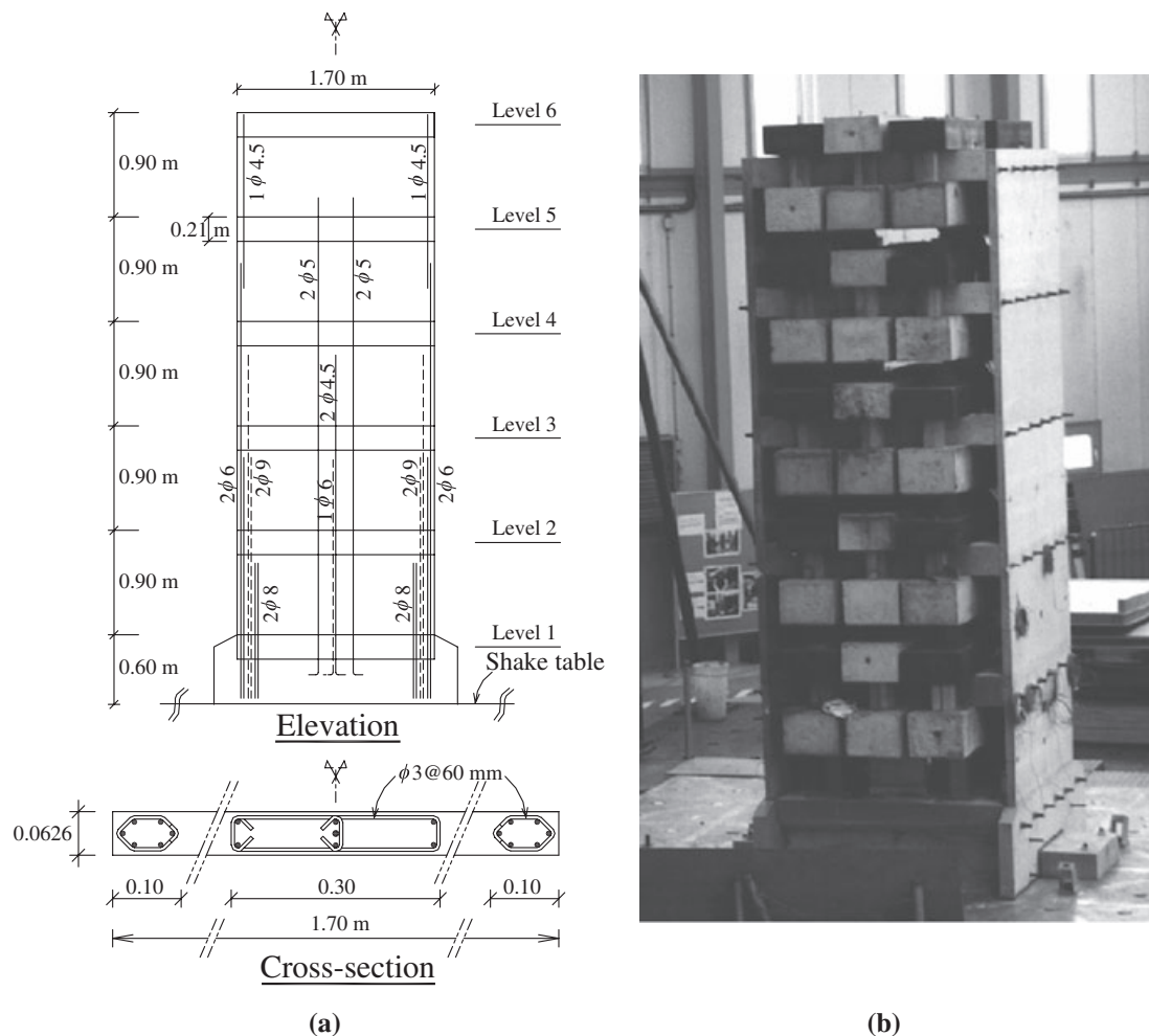
Figure 1. CAMUS test walls (CEA, 2002): (a) details of reinforcement; (b) final test set-up
