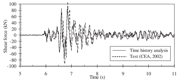
(c) Shear force at level 1
