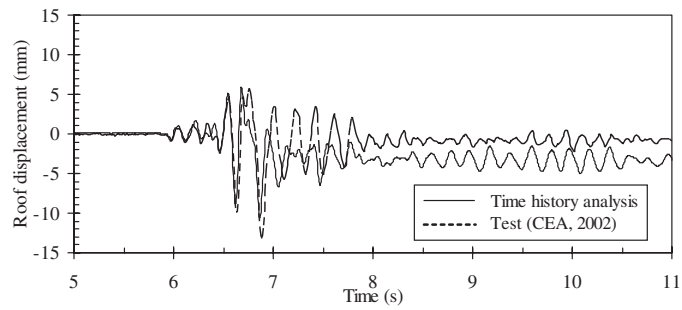
(a) Top floor lateral displacement response
