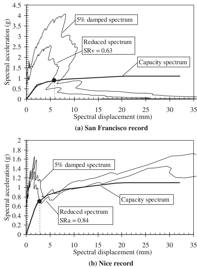
Figure 14. Performance point representation to evaluate the top-floor displacement of the wall when subjected to San Francisco and Nice records
