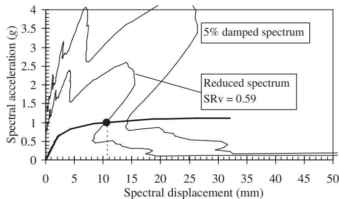
Figure 10. Response spectra to 15 mm performance for San Francisco record (PGA 1.30 g)
