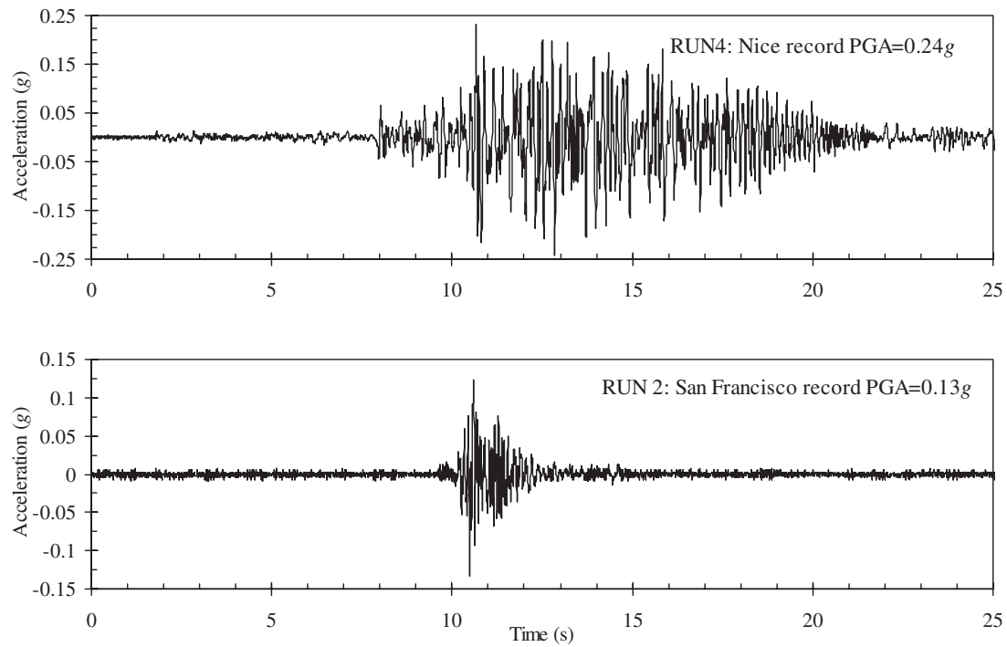
Figure 2. Measured accelerations on top of the shake table for the analysed runs (CEA, 2002)
