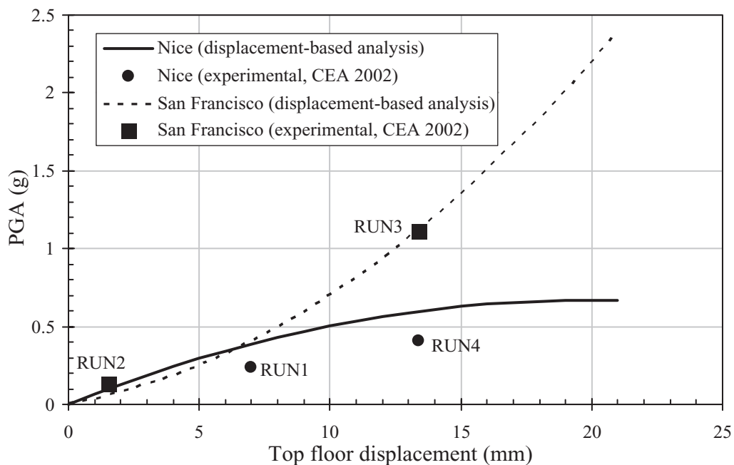
Figure 11. Estimated PGA at target top-floor displacements from the displacement-based approach versus results of the four tests of CEA, 2002
