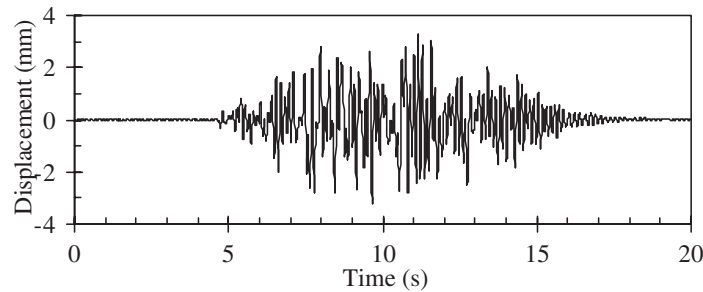
(b) Nice record
