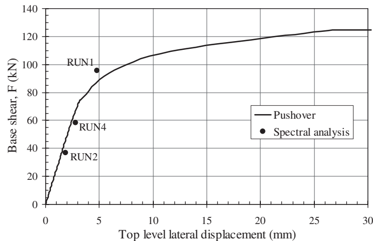
Figure 6. Nonlinear pushover analysis force-displacement relationship
