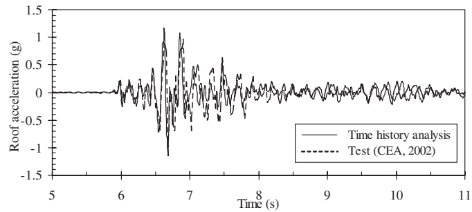
(b) Top floor lateral acceleration
