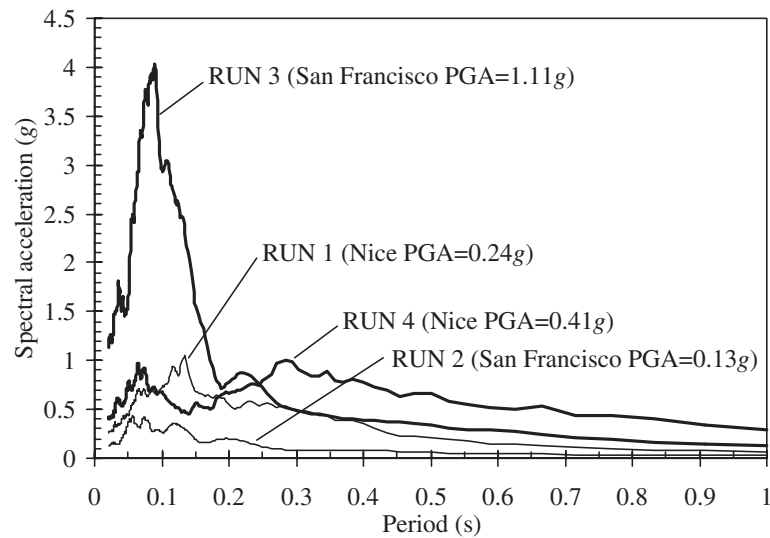
Figure 3. Response spectra for the four experimental runs
