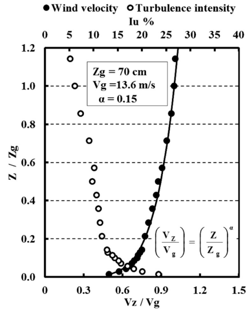
Fig. 2. Wind velocity and turbulence intensity profiles for open terrain exposure.
