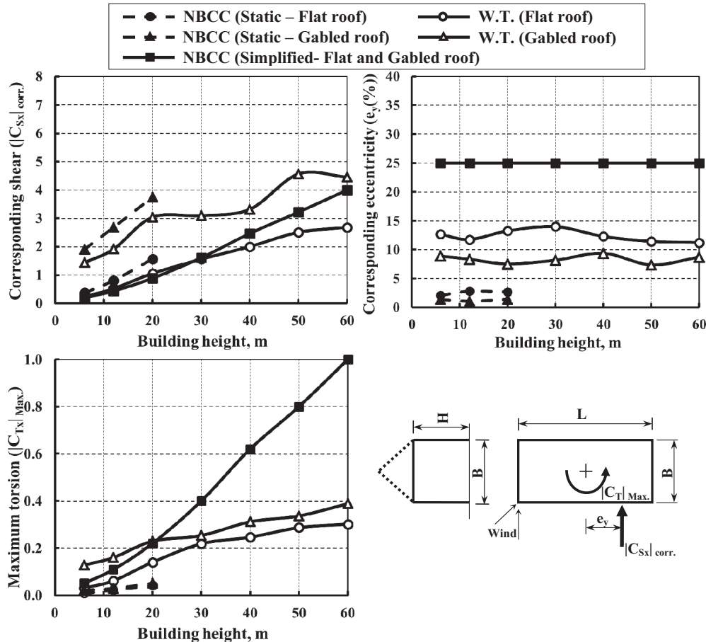
Fig. 9. Comparison of torsional load case evaluated using NBCC 2010 and wind tunnel measurements for buildings with 0° and 45° roof angles (Transverse direction).
