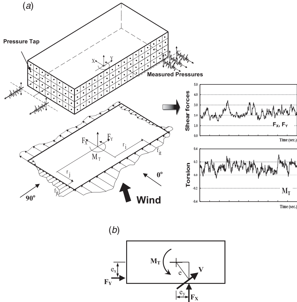
Fig. 3. (a) Measurement procedure for horizontal wind forces, F_x and F_y , and torsional moment, M_T ; (b) resultant and wind force components along with the eccentricities in transverse (x) and longitudinal (y) directions.
