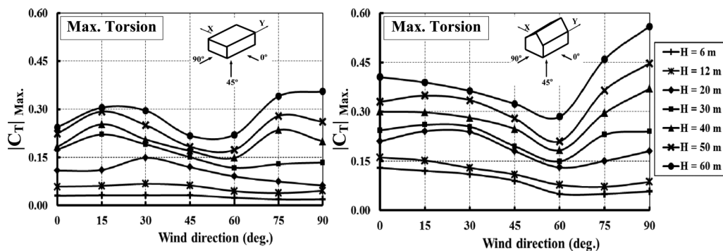
Fig. 4. Variation of peak torsion coefficient ( |C_T|_{Max} ) with wind direction for the tested buildings with flat and gabled roof.
