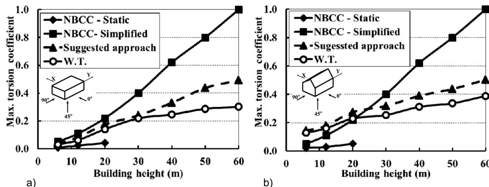
Fig. 13. Maximum torsion evaluated using NBCC 2010, wind tunnel measurements and suggested approach in transverse direction for buildings with: (a) flat roof and (b) gabled roof.
