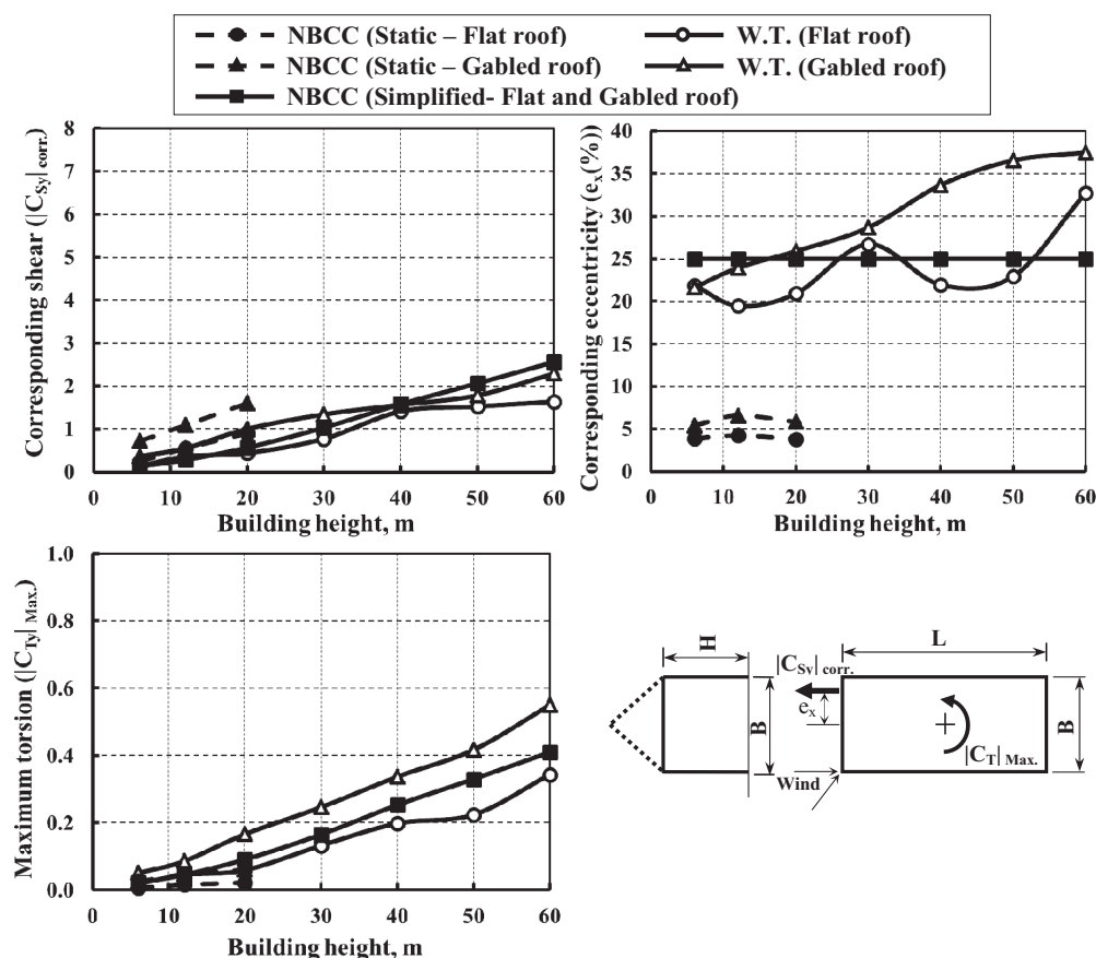
Fig. 11. Comparison of torsional load case evaluated using NBCC 2010 and wind tunnel measurements for buildings with 0° and 45° roof angles (longitudinal direction).
