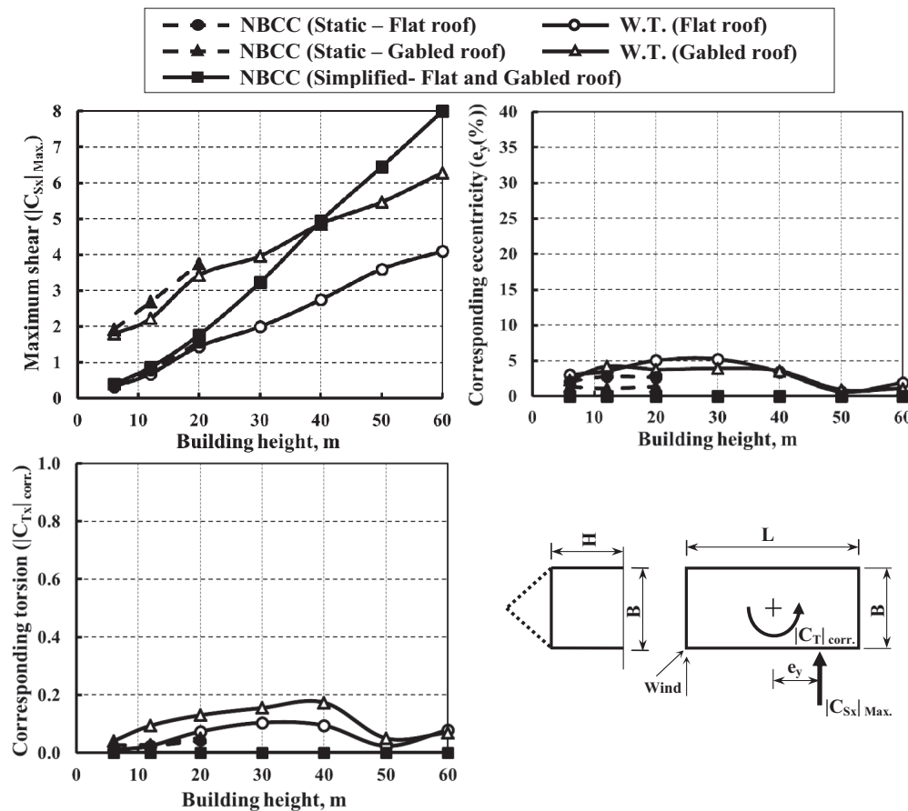
Fig. 10. Comparison of shear load case evaluated using NBCC 2010 and wind tunnel measurements for buildings with 0° and 45° roof angles (Transverse direction).
