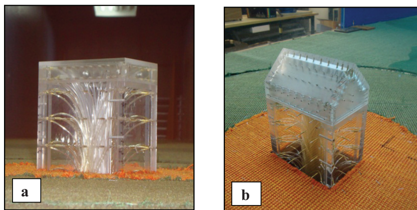
Fig. 1. Wind tunnel models: (a) building with a flat roof ( 0^\circ ) and (b) building with a gabled-roof ( 45^\circ ).
