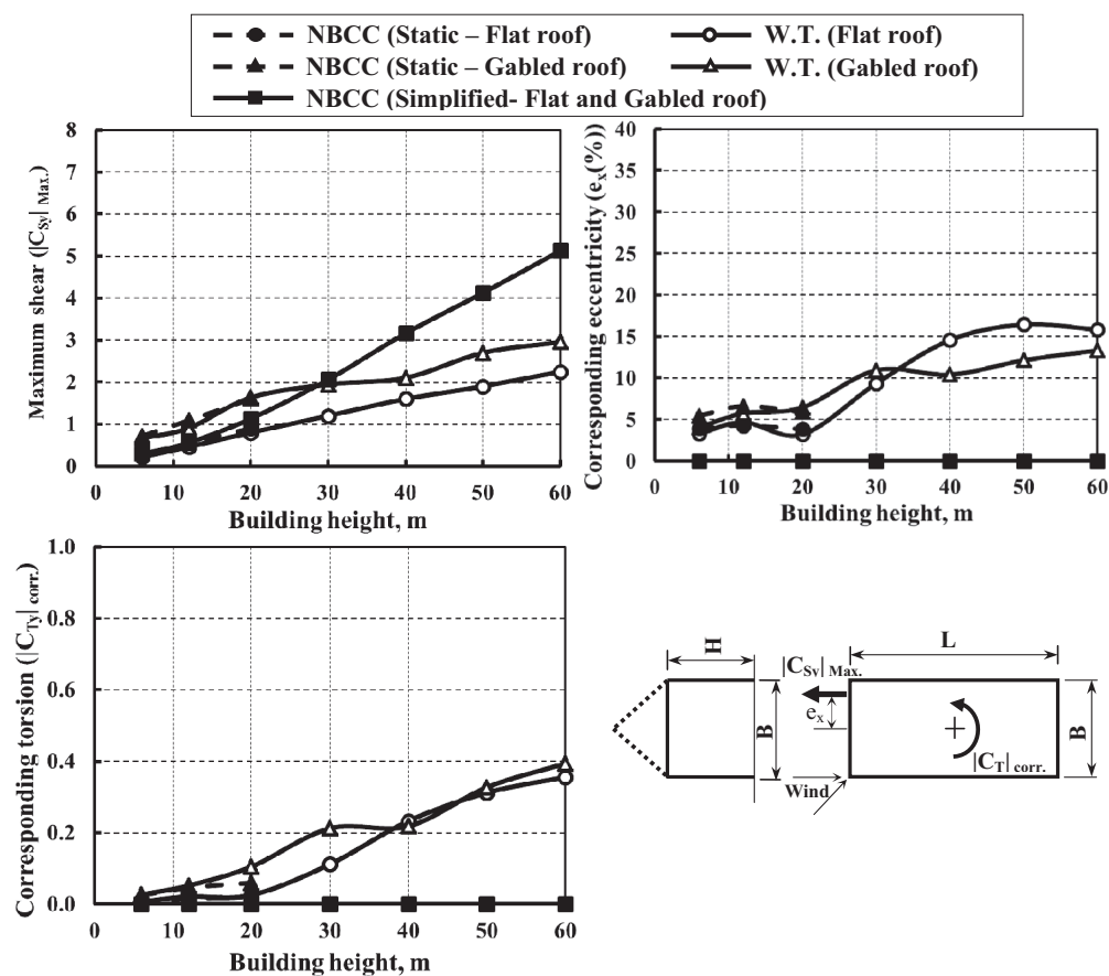
Fig. 12. Comparison of shear load case evaluated using NBCC 2010 and wind tunnel measurements for buildings with 0° and 45° roof angles (longitudinal direction).
