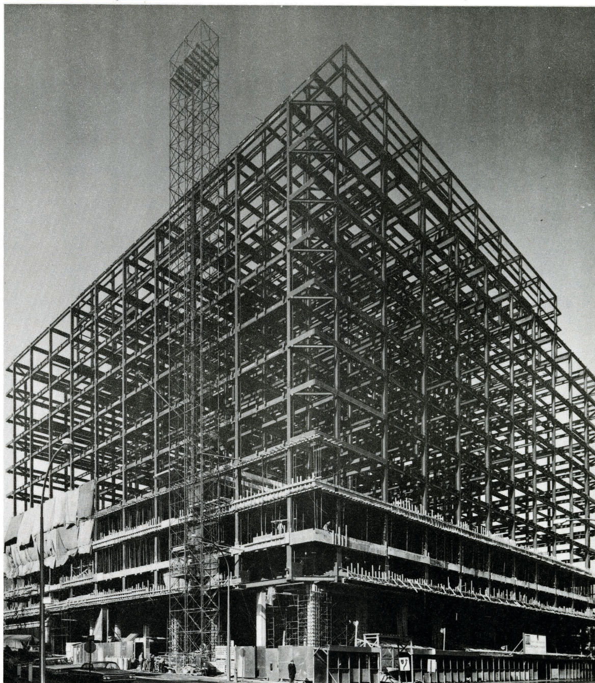
HENRY F. HALL BUILDING Sir George Williams University Montreal Quebec
